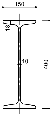
400 × 150 × 10 × 18 (72.0kg/m)
