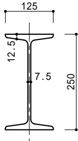
250 × 125 × 7.5 × 12.5 (38.3kg/m)
