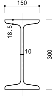
300 × 150 × 10 × 18.5 (65.5kg/m)
