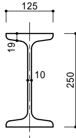
250 × 125 × 10 × 19 (55.5kg/m)
