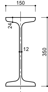
350 × 150 × 12 × 24 (87.2kg/m)
