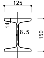
150 × 125 × 8.5 × 14 (36.2kg/m)
