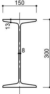
300 × 150 × 8 × 13 (48.3kg/m)
