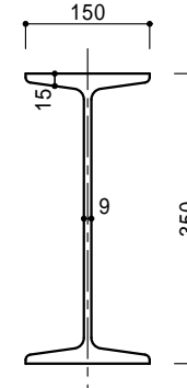
350 × 150 × 9 × 15 (58.5kg/m)
