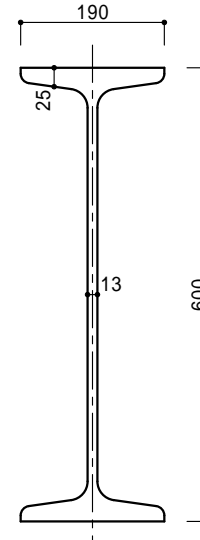
600 × 190 × 13 × 25 (133kg/m)
