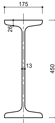
450 × 175 × 13 × 26 (115kg/m)
