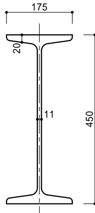
450 × 175 × 11 × 20 (91.7kg/m)
