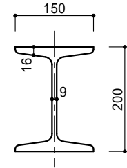
200 × 150 × 9 × 16 (50.4kg/m)
