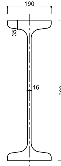
600 × 190 × 16 × 35 (176kg/m)
