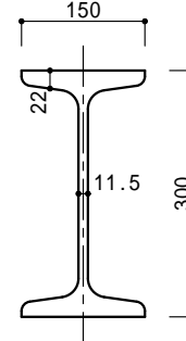
300 × 150 × 11.5 × 22 (76.8kg/m)
