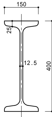
400 × 150 × 12.5 × 25 (95.8kg/m)
